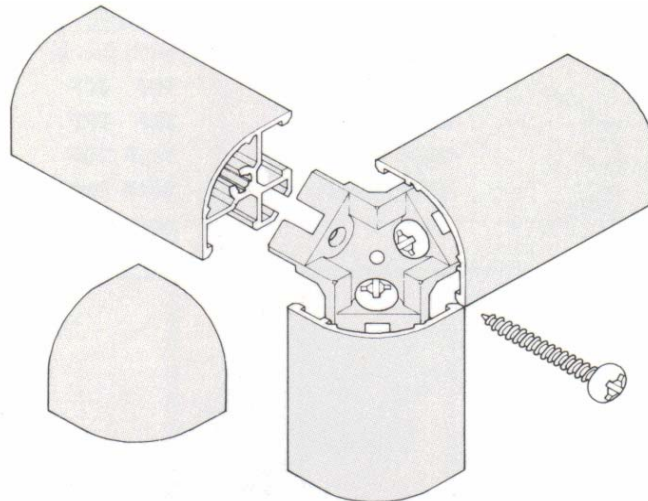
Example QS corner construction detail
